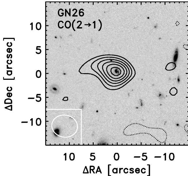
FIG. 1.—Integrated CO(2→1) map of GN 26 averaged over 312.5 MHz ( 904 \text{ km s}^{-1} ) overlaid on an optical HST ACS z -band image (gray scale). The 1 \sigma error is 0.46 \text{ Jy km s}^{-1} \text{ beam}^{-1} , and the contour levels are 1 \sigma \times (-2, 2, 3, 4, 5, 6, 7) ; positive contours are solid lines and negative contours are dotted lines. The synthesized beam size (white ellipse) for the observations is shown in the lower left ( 5.4'' \times 4.6'' , P.A. = 80^\circ ).
