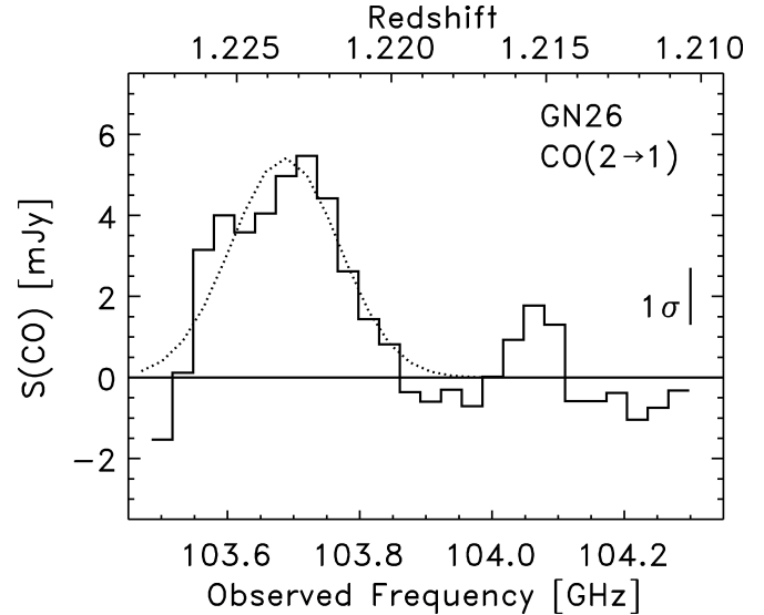
FIG. 2.—CO(2→1) spectrum for GN 26. The spectrum has been Hanning-smoothed. The channel increment is 31.25 \text{ MHz} ( 90.4 \text{ km s}^{-1} ), and the 1 \sigma error bar per smoothed channel is shown to the right. The dotted line shows a Gaussian fit of the line profile for the unsmoothed data.
