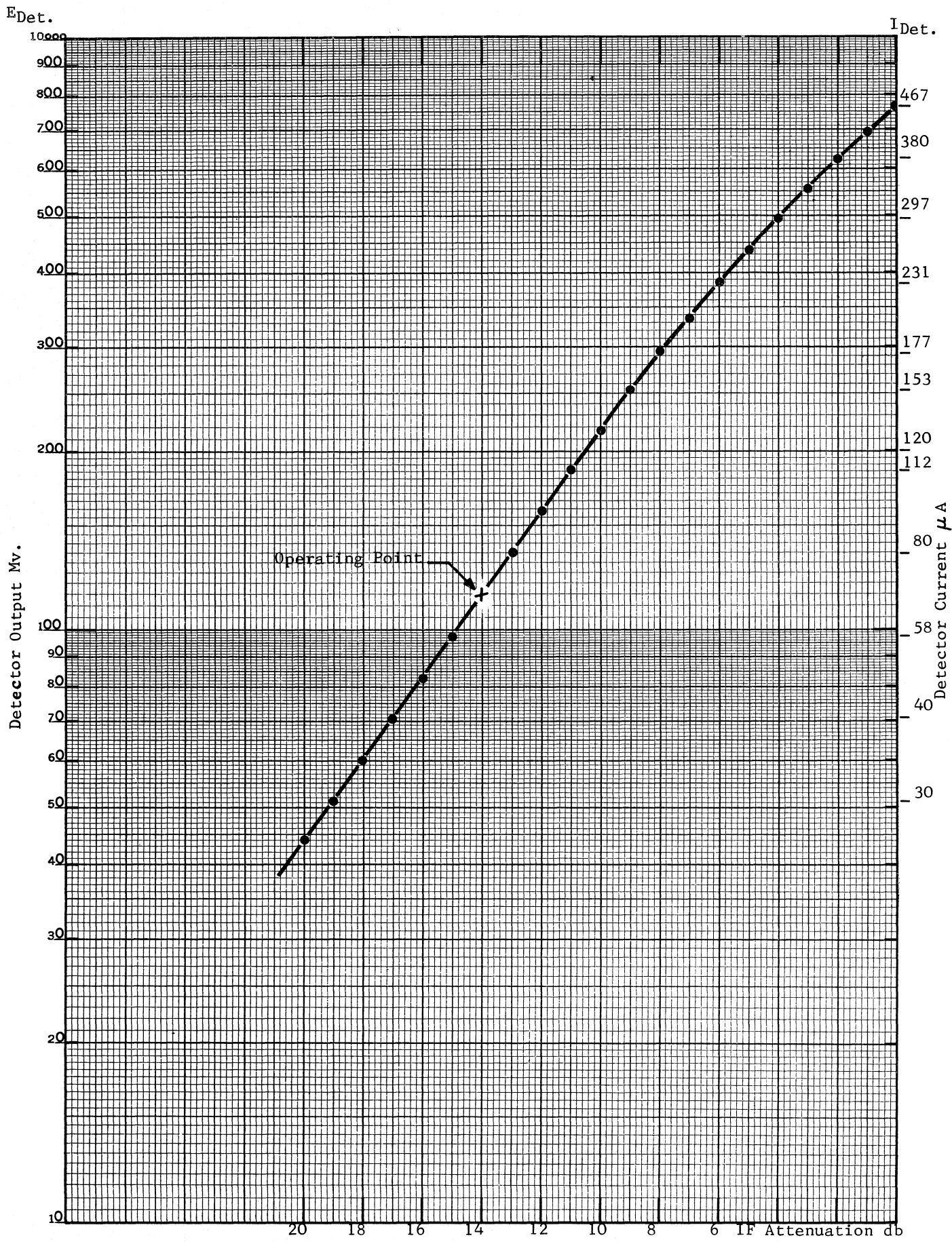
FIG. 6. BACK END DETECTOR CHARACTERISTIC
