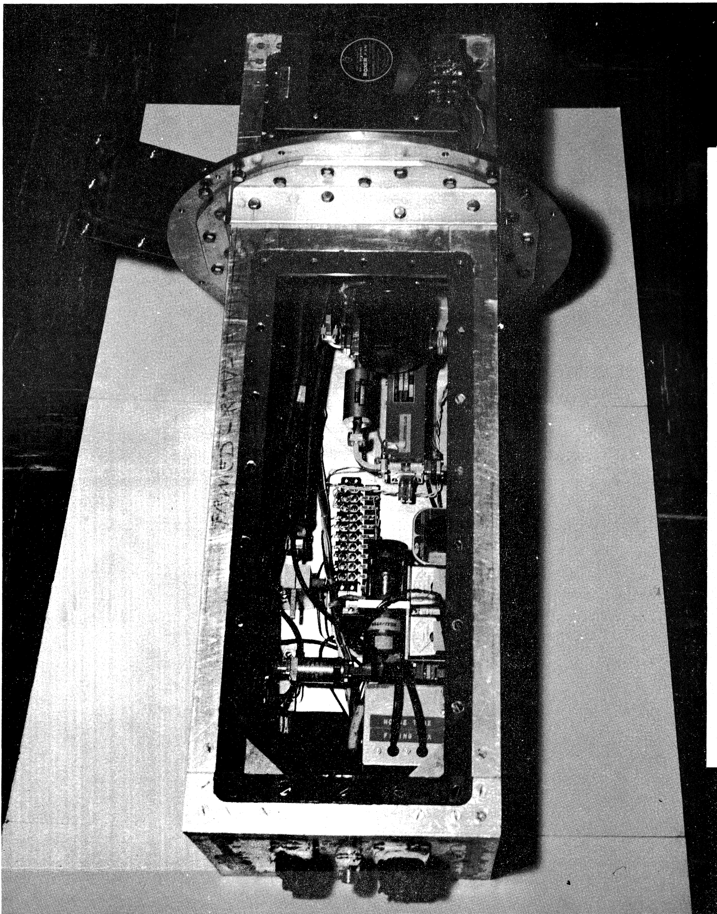
FIG. 12. PACKAGED FRONT END IN STANDARDIZED TEMPERATURE CONTROLLED BOX
