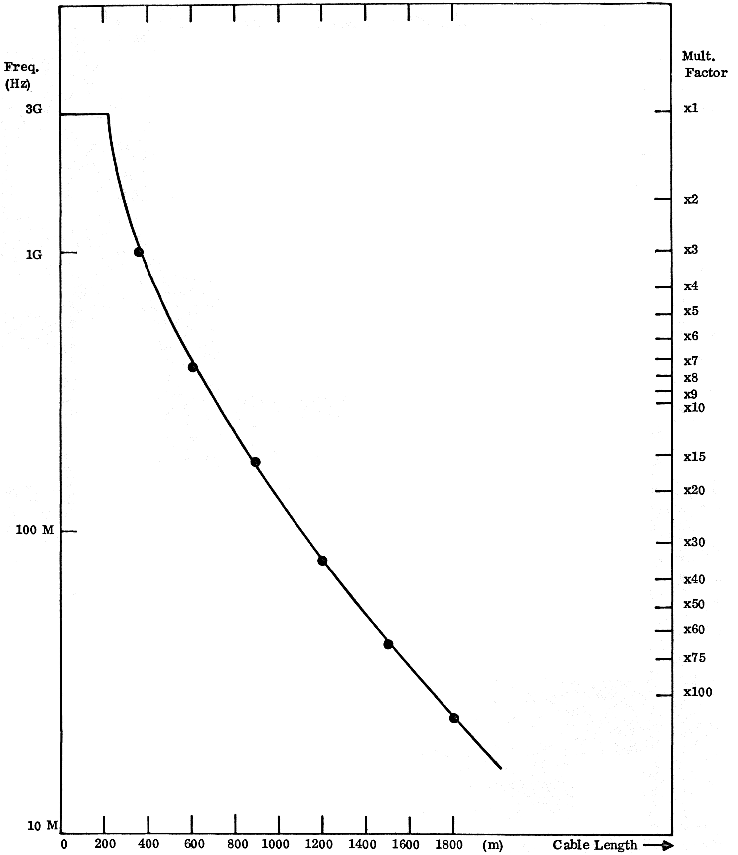
FIG. 3 - MINIMUM TOTAL LOSS TRANSMISSION FREQUENCY VS. CABLE LENGTH FOR PRODELIN SPIROLINE 1 5/8", 50 OHM CABLE
