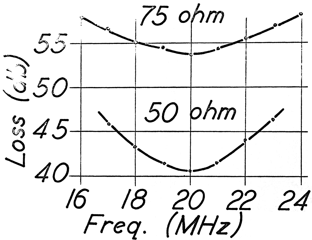
Figure 2. Performance of a 1 ms delay line shown above to illustrate the effect of impedance on bandwidth and insertion loss.
