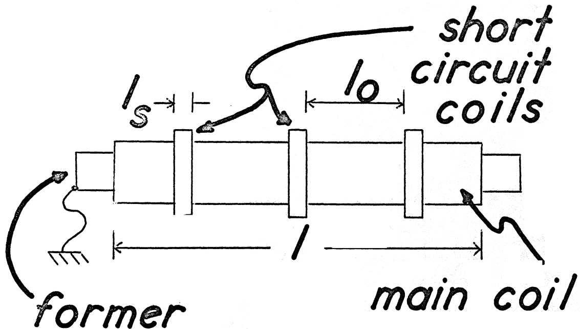
Figure 5 (b). Construction of the Delay Line.
