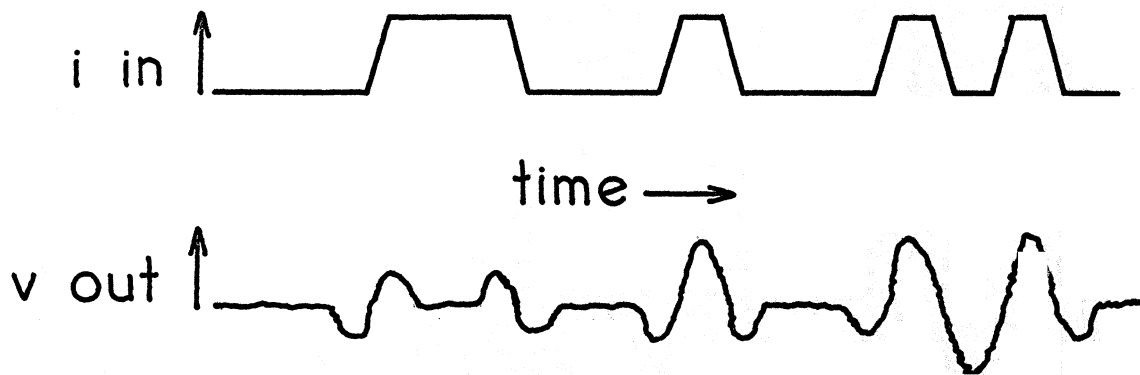
Figure 8. Waveforms associated with longitudinal mode magnetostrictive delay line.
