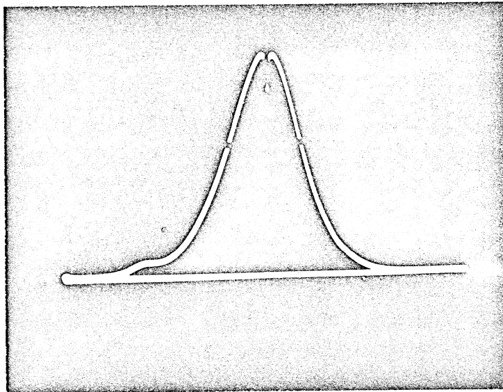
Figure 20. Typical frequency response of 234 MHz and 256 MHz systems. Bandwidth 4 MHz.
