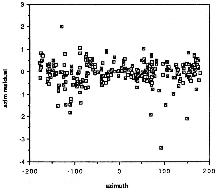
45-ft feb 8: azimuth residuals vs az
