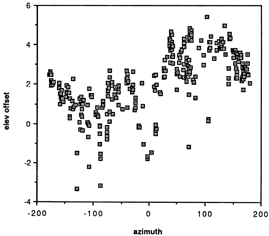
elevation offset vs azimuth
