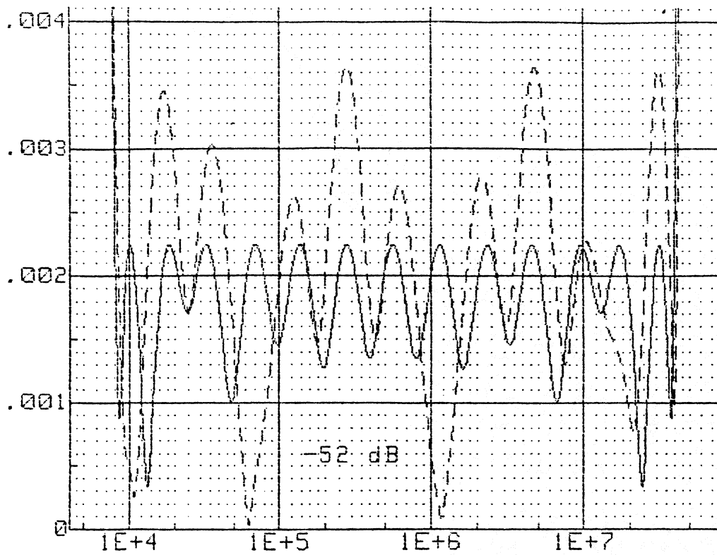
Figure 2 Theoretical Image Response of SSB Demodulator.
