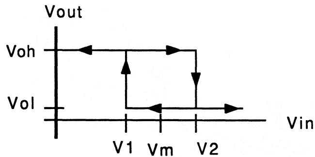
Figure 4 Comparator Transfer Function
