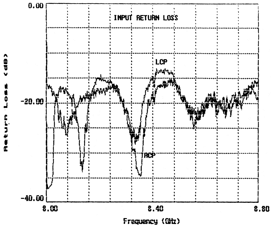
S/X DEMAR, SN 03, X-BAND 3/23/89
