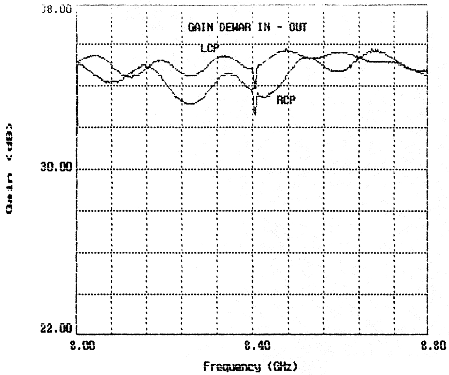
S/X DEWAR, SN 03, X-BAND 3/23/89
