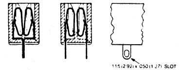
Solder Eyelet
