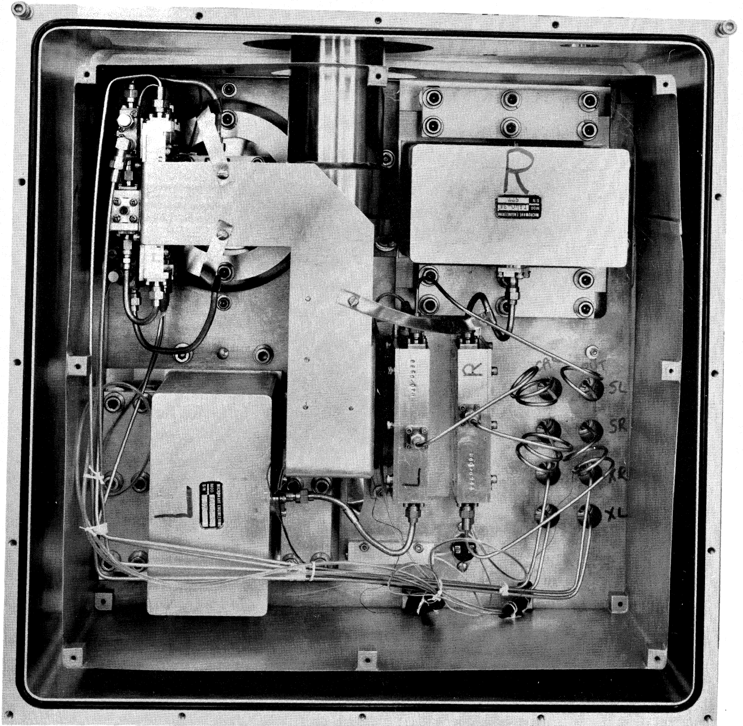
FIGURE 3 Dewar Interior
