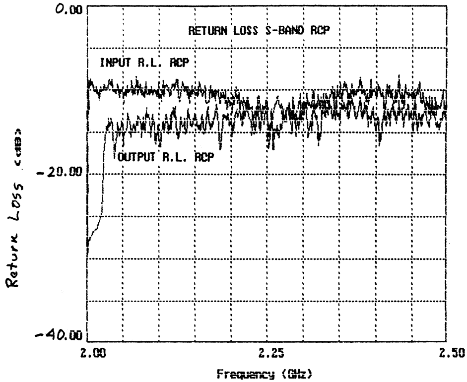
S/X DEMAR, SN 03, S-BAND 3/22/89
