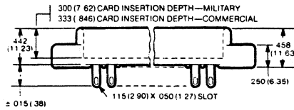
With plain mounting holes
