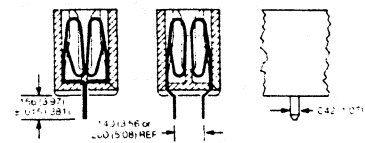
Dip Solder
