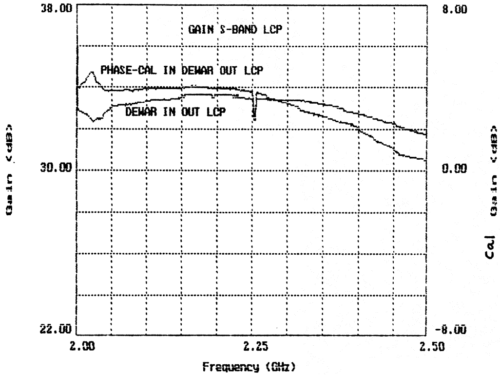
S/X DEWAR, SN 03, S-BAND 3/22/89
