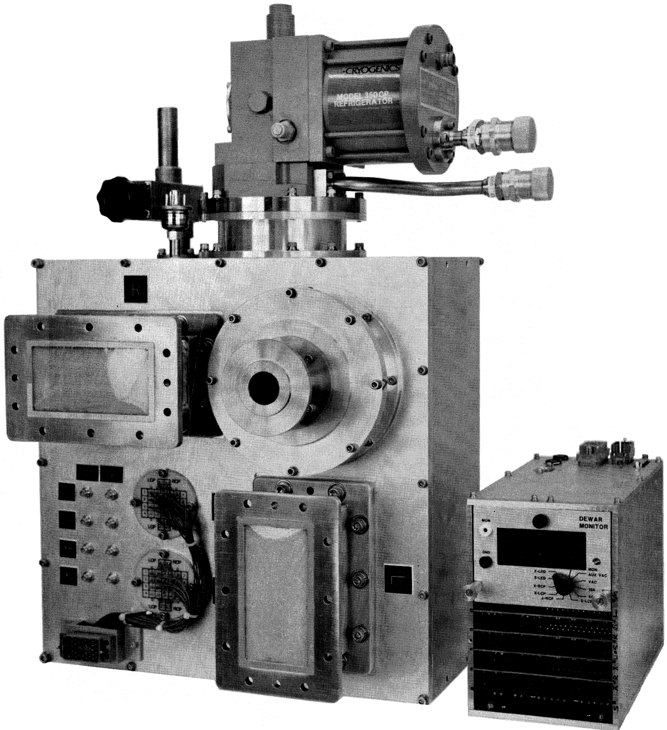
FIGURE 1 S/X Dewar Assembly
