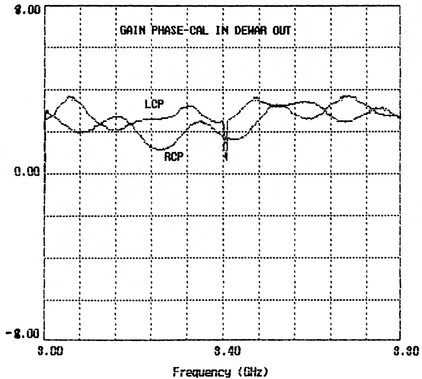
S/X DEWAR, SN 03, X-BAND 3/23/89
