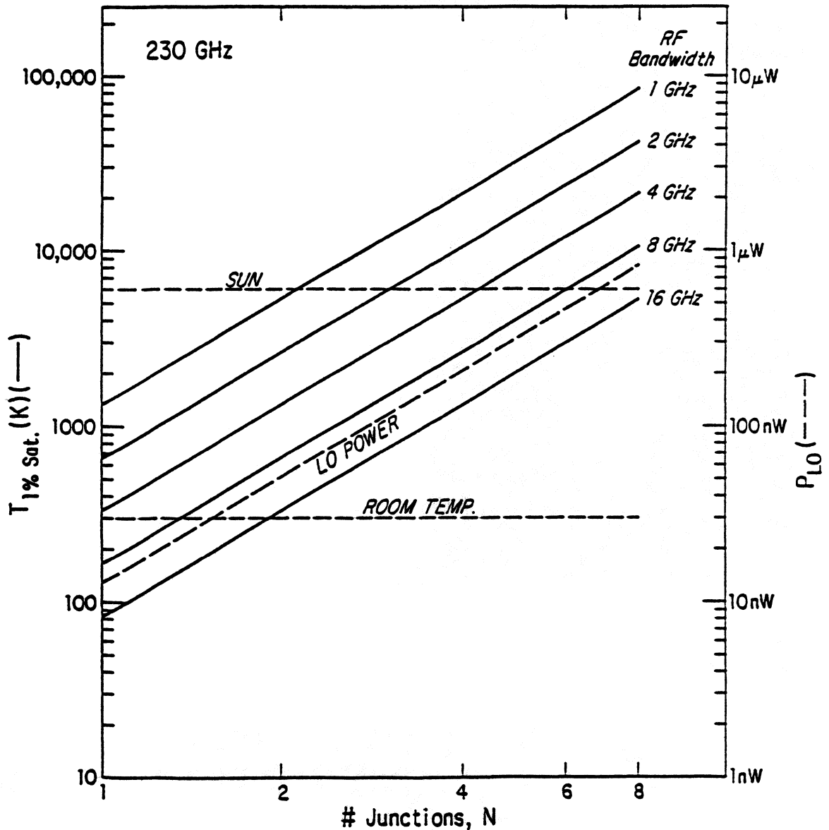
Fig. 3. Thermal source temperature to give 1% gain compression in a 230 GHz SIS mixer as a function of the number of junctions N , for various RF bandwidths. Also shown is the LO power as a function of N . Other parameters assumed in calculating T_{\text{sat}} from eqn.(17) are L = 0.0 \text{ dB} and R_L = 50 \Omega . Other parameters assumed in calculating P_{LO} from eqn.(10) are \alpha = 1.2 and R_{n,\text{array}} = 50 \Omega .
