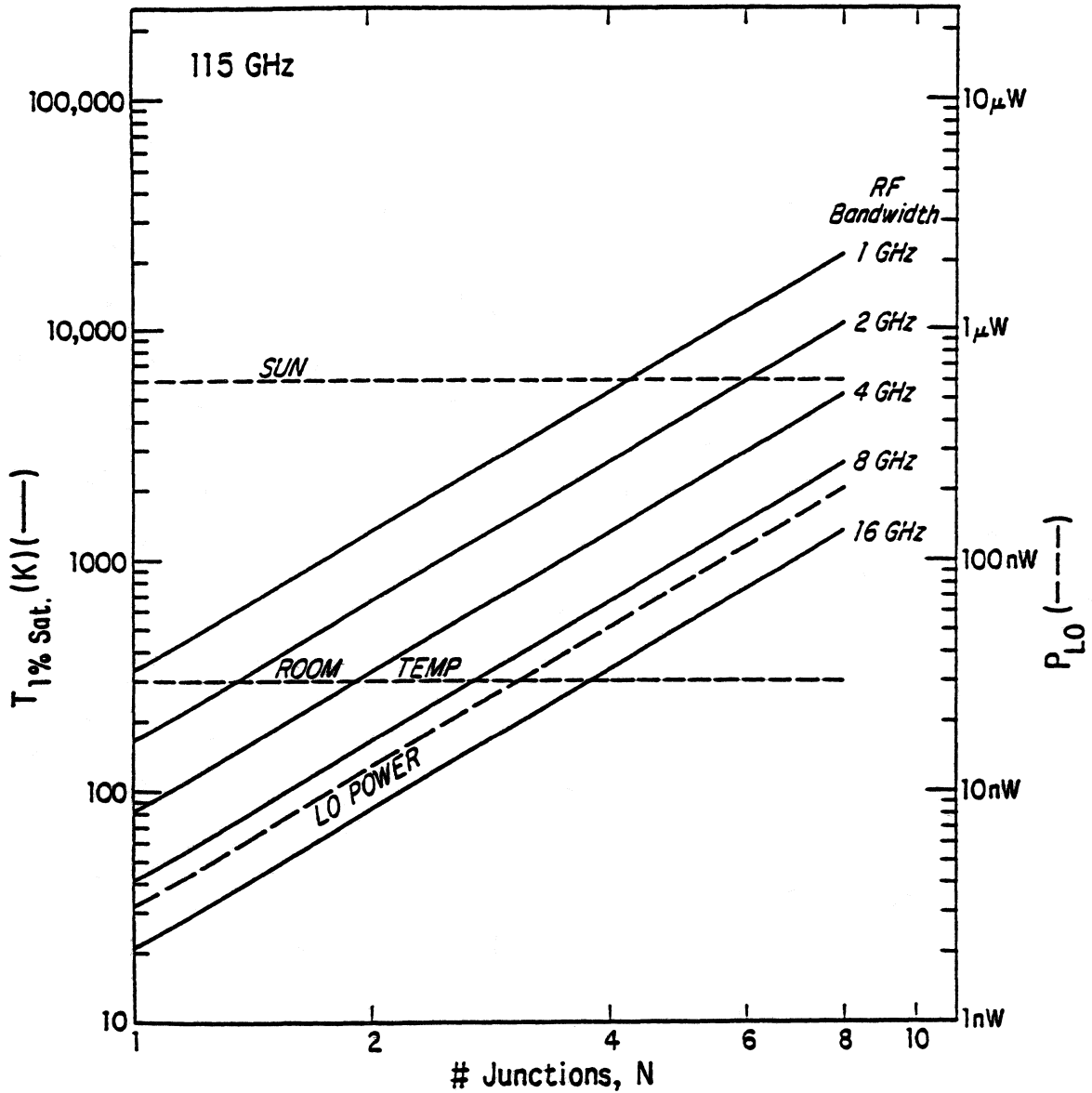
Fig. 2. Thermal source temperature to give 1% gain compression in a 115 GHz SIS mixer as a function of the number of junctions N , for various RF bandwidths. Also shown is the LO power as a function of N . Other parameters assumed in calculating T_{\text{sat}} from eqn.(17) are L = 0.0 \text{ dB} and R_L = 50 \Omega . Other parameters assumed in calculating P_{LO} from eqn.(10) are \alpha = 1.2 and R_{N,\text{array}} = 50 \Omega .
