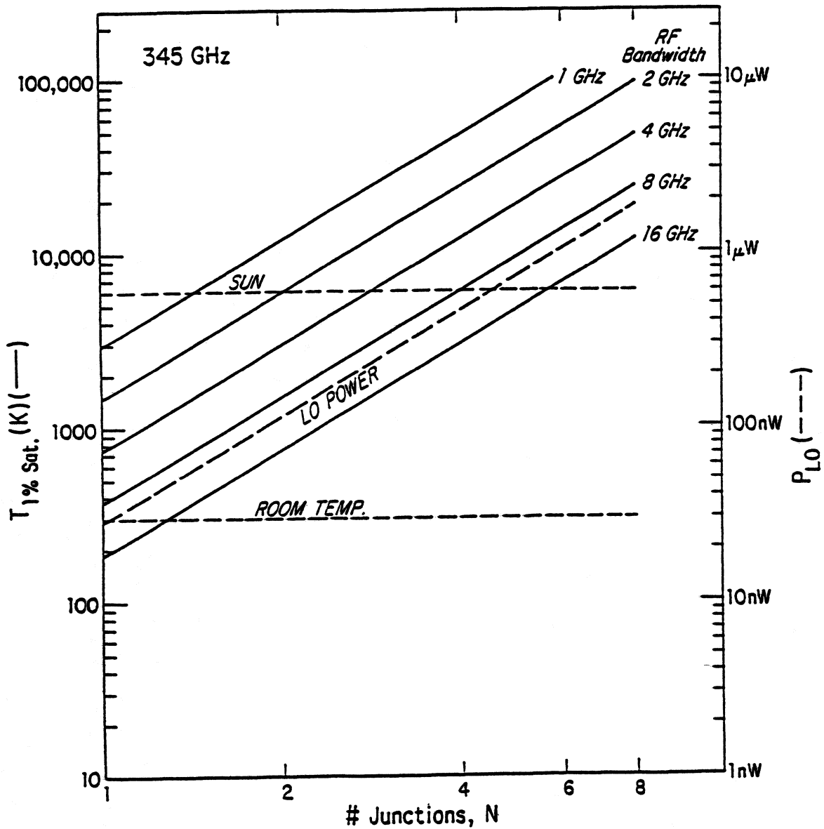
Fig. 4. Thermal source temperature to give 1% gain compression in a 345 GHz SIS mixer as a function of the number of junctions N , for various RF bandwidths. Also shown is the LO power as a function of N . Other parameters assumed in calculating T_{\text{sat}} from eqn.(17) are L = 0.0 \text{ dB} and R_L = 50 \Omega . Other parameters assumed in calculating P_{LO} from eqn.(10) are \alpha = 1.2 and R_{n,\text{array}} = 50 \Omega .
