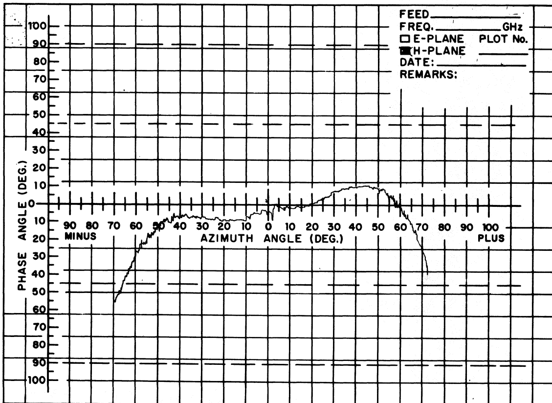
Figure 7. Typical Amplitude and Phase Patterns at 14 GHz with the YIG Tuned Multiplier Signal Source.
