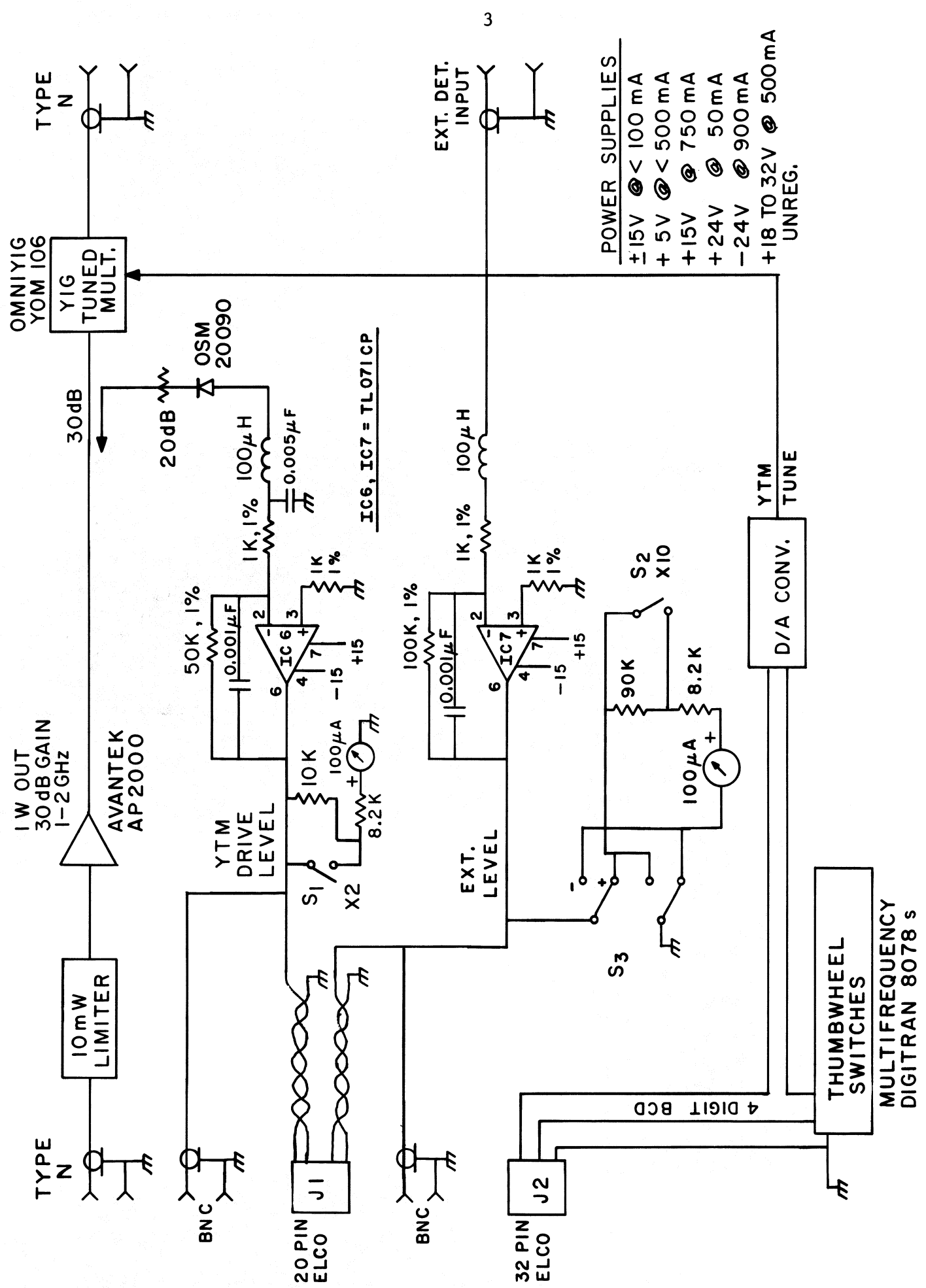
Figure 1. 2 to 18 GHz Multiplier Chassis Circuit (transmitter tower).
