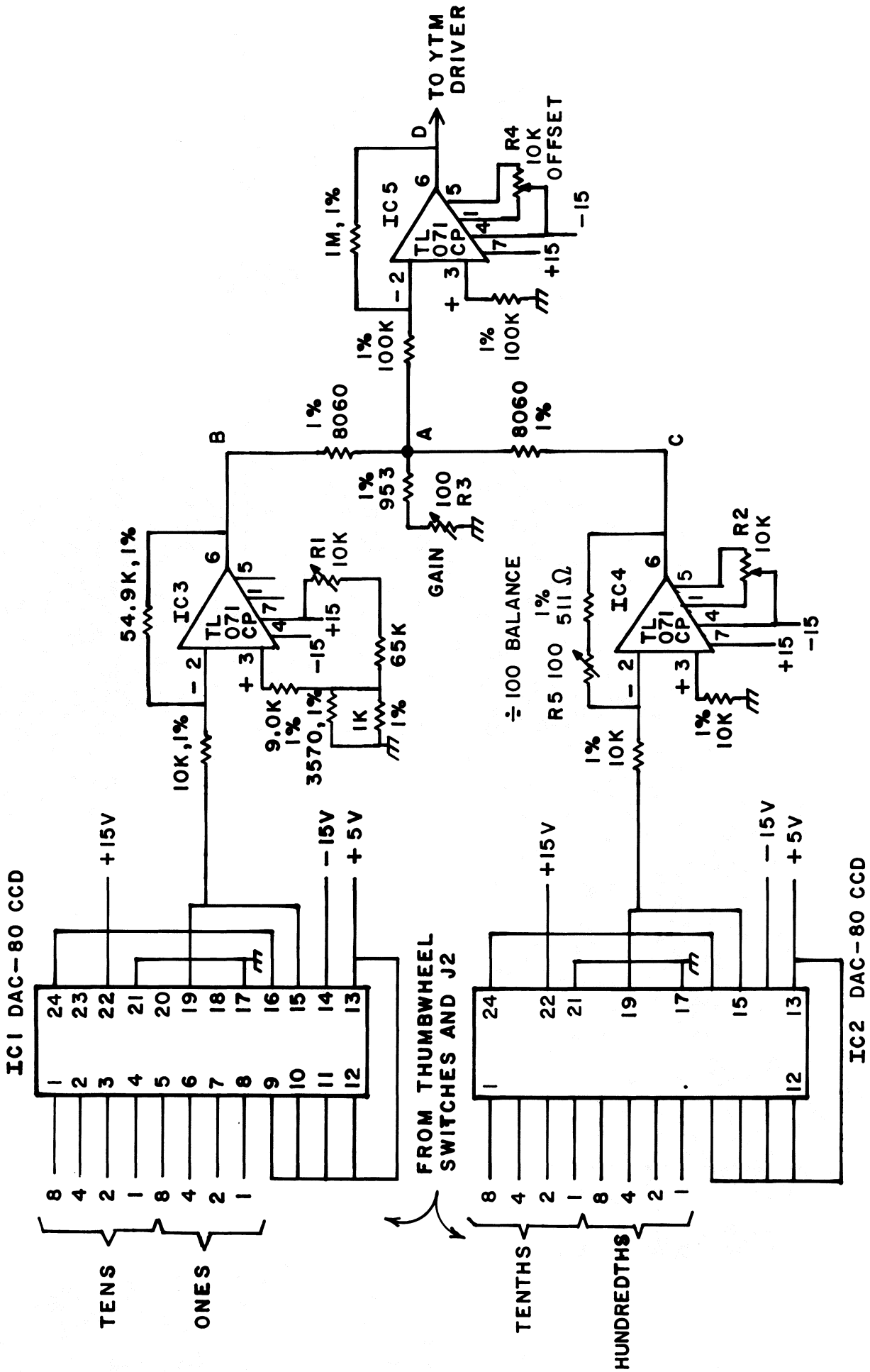
Figure 3. D/A Converter Circuits for the YIG Tuned Multiplier Frequency Control (transmitter tower).
