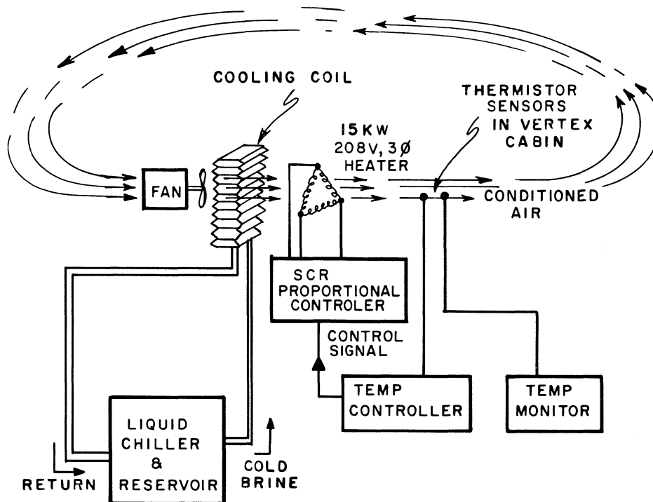
TEMP. CONTROL SYSTEM BLOCK DIAGRAM
