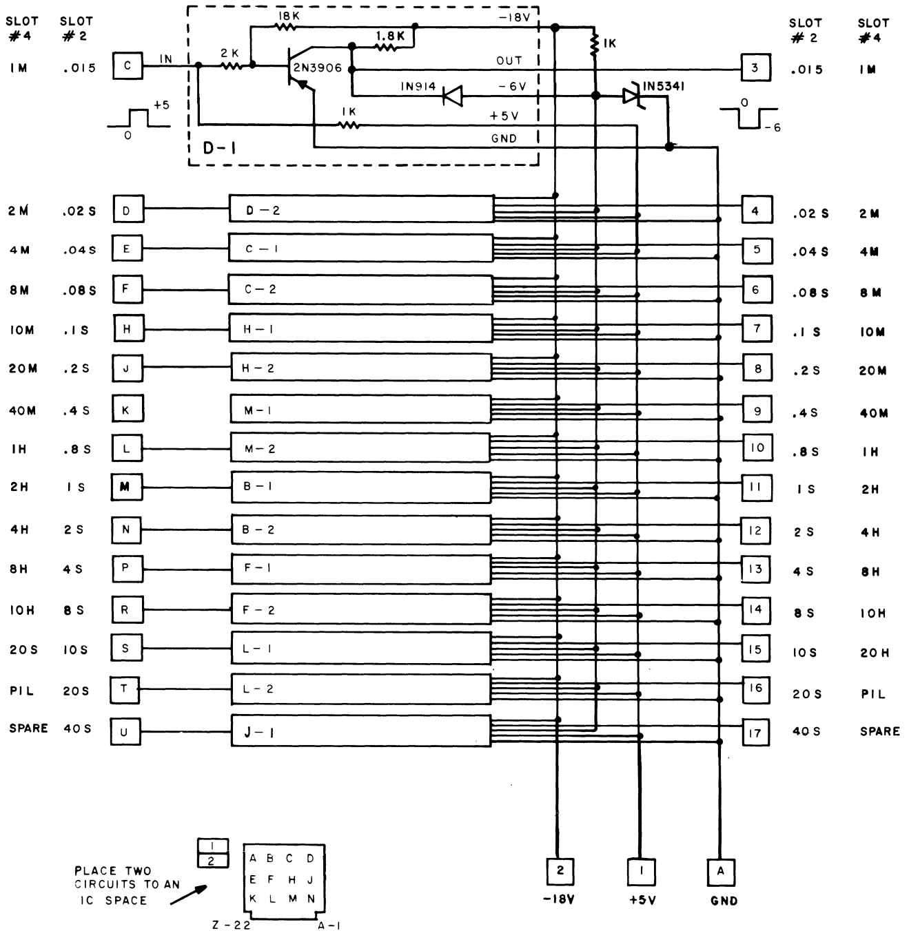
NRAO STANDARD TIME CLOCK COMPUTER BUFFER CARD # 2/4 FIG.
