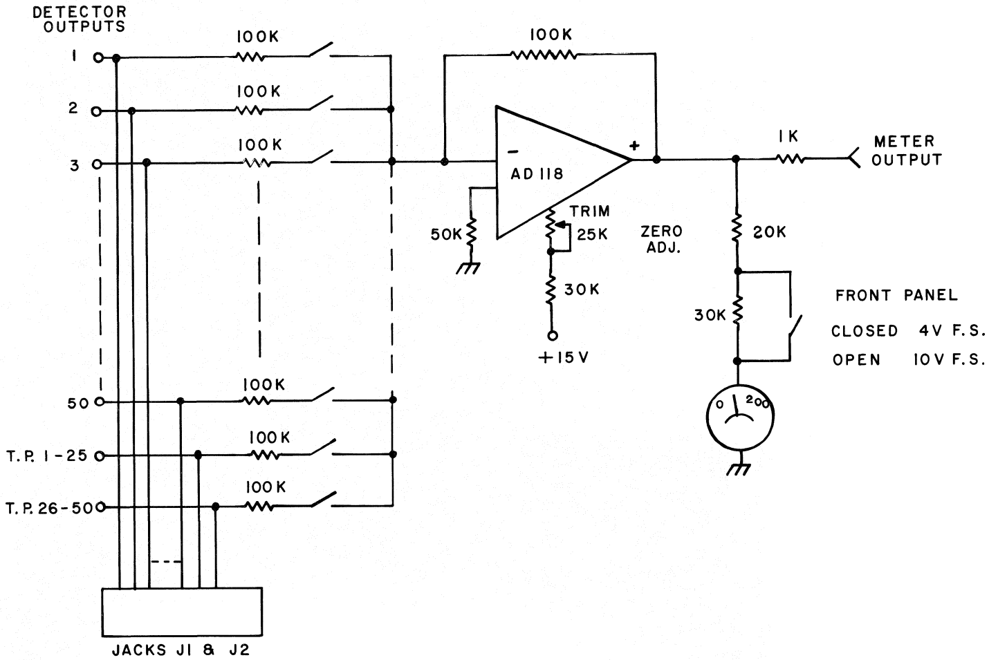
Figure 6 Meter amplifier circuit.
