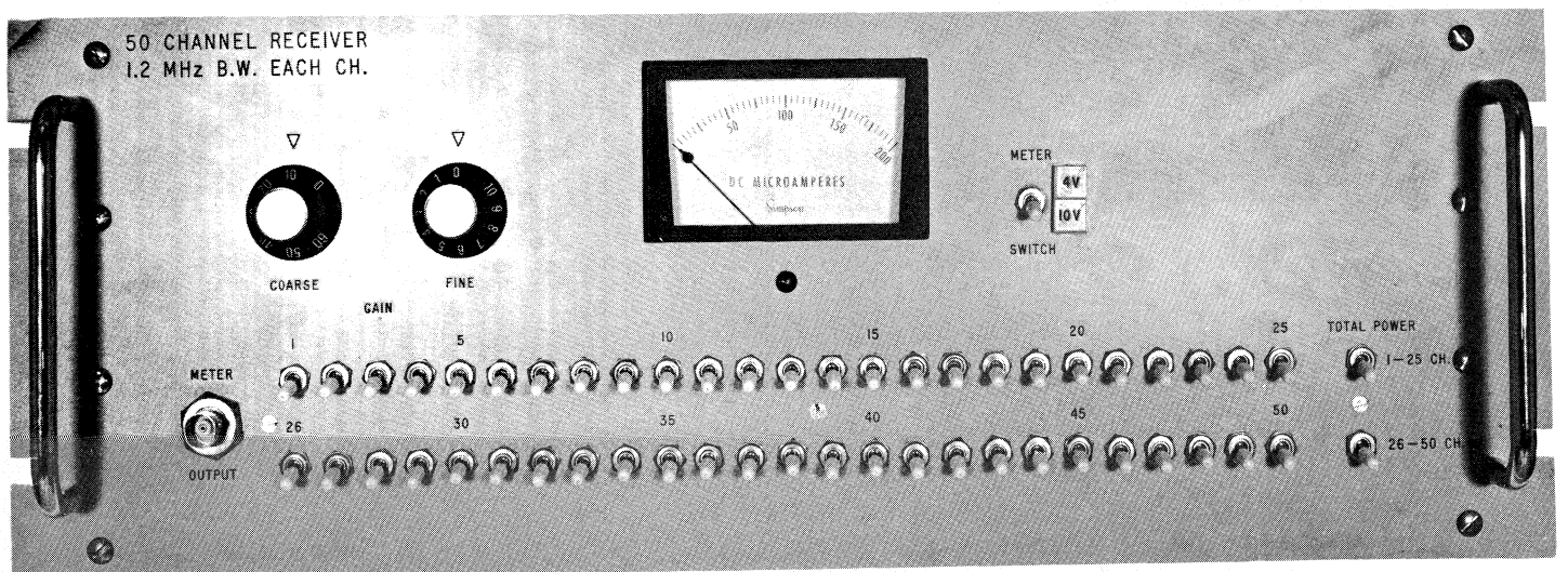
Figure 2 Front panel and top view of the receiver.
