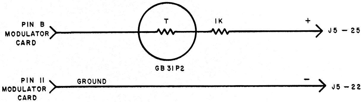
TEMPERATURE CIRCUIT IN WAYNE GEORGE ELECTRONICS BOX SCHEMATIC # 18
