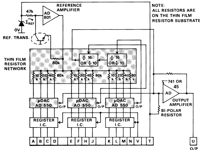
Fig. 1. Block Diagram of DAC-Q
