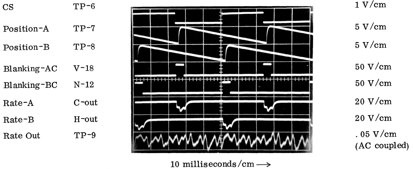
Figure 9 — Principal Analog Signals present in the Analog Card with Constant Rate Equal to 26°/minute.
