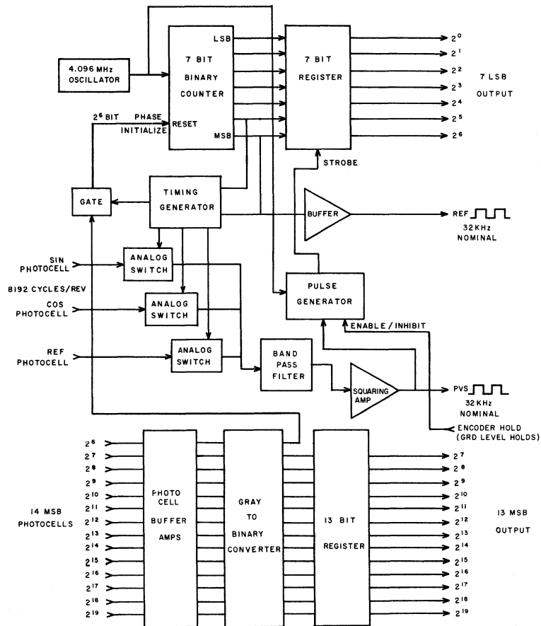
BALDWIN MODEL 694BL ENCODER BLOCK DIAGRAM
