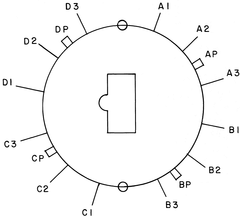
FRONT VIEW (KNOB END)
