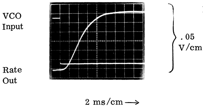
Figure 10 — Rate Step Response
