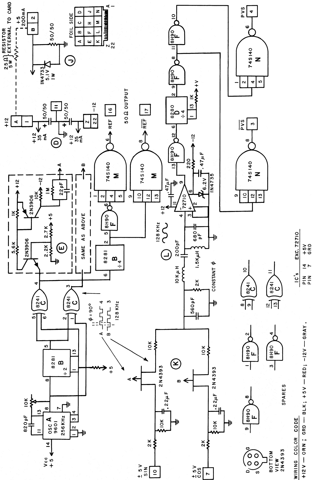
W / G TO BALDWIN MODULATOR CARD SCHEMATIC # 7
