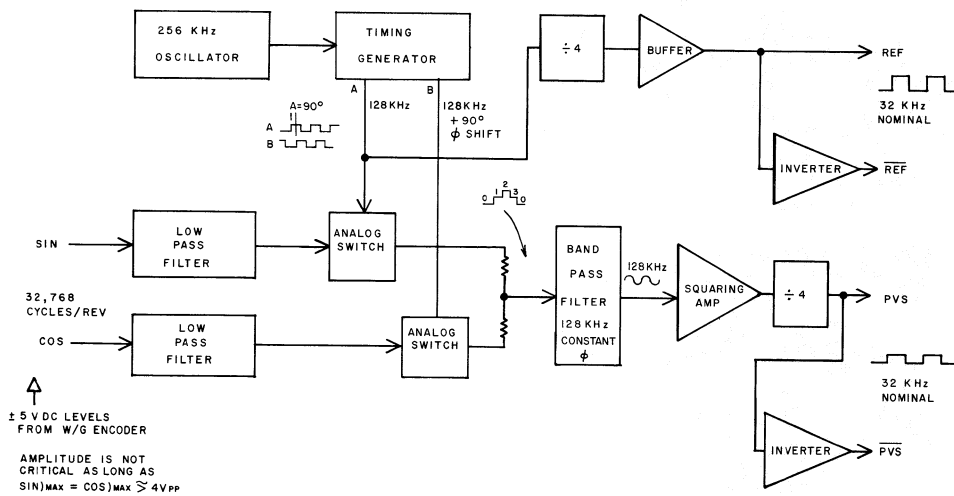
W/G TO BALDWIN FORMAT CONVERTER CARD
