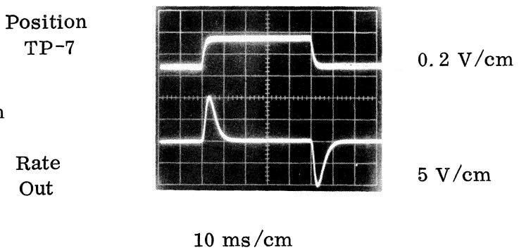
Figure 11 — Rate Impulse Response
