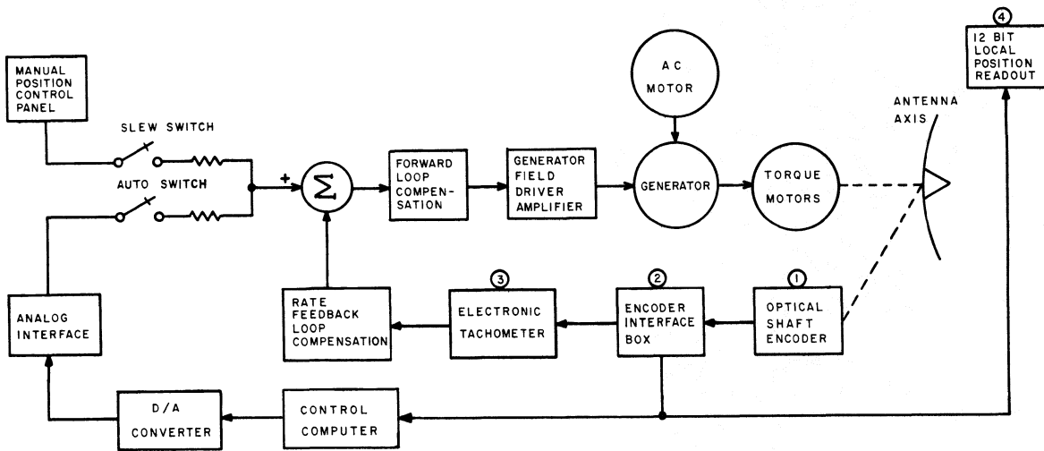
SIMPLIFIED BLOCK DIAGRAM OF POSITION CONTROL SYSTEM
