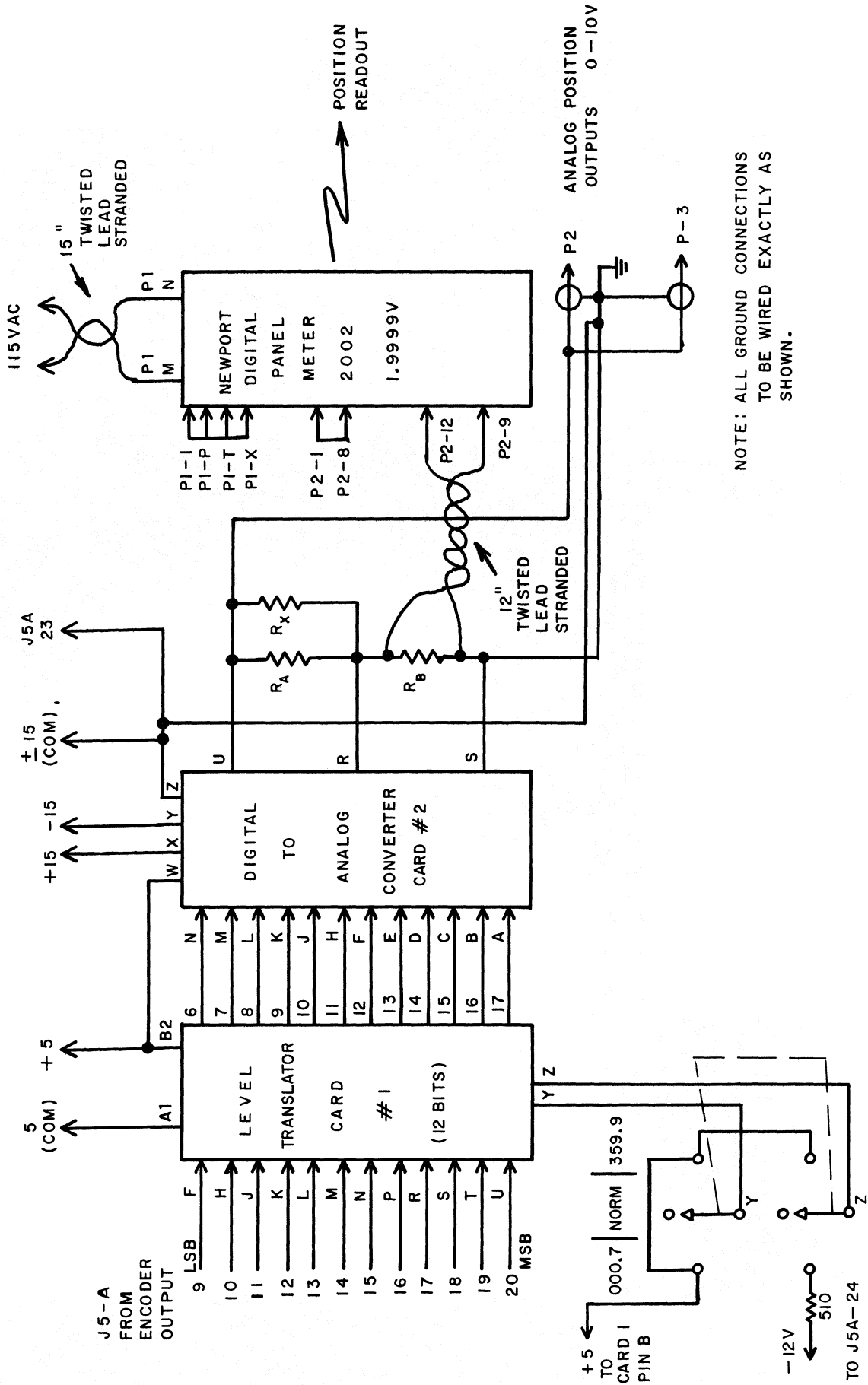
LOCAL POSITION READOUT AZIMUTH SCHEMATIC # 11
