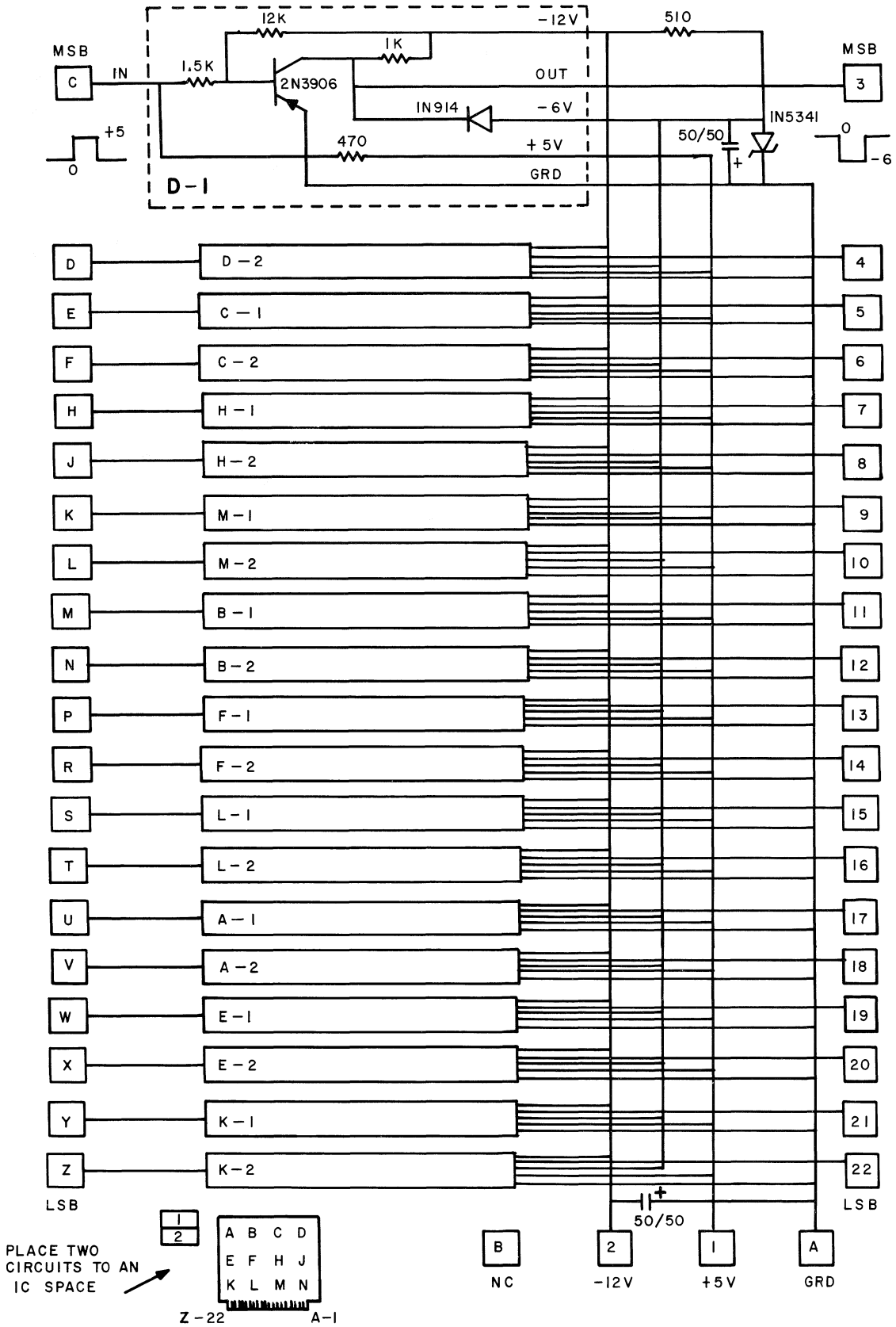
DATA OUTPUT TO COMPUTER BUFFER CARD # 1 SCHEMATIC # 2
