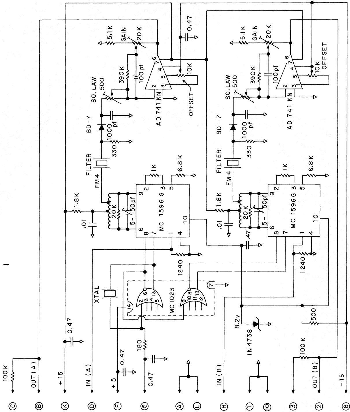
DUAL FILTER CIRCUIT BOARD FIG. 3
