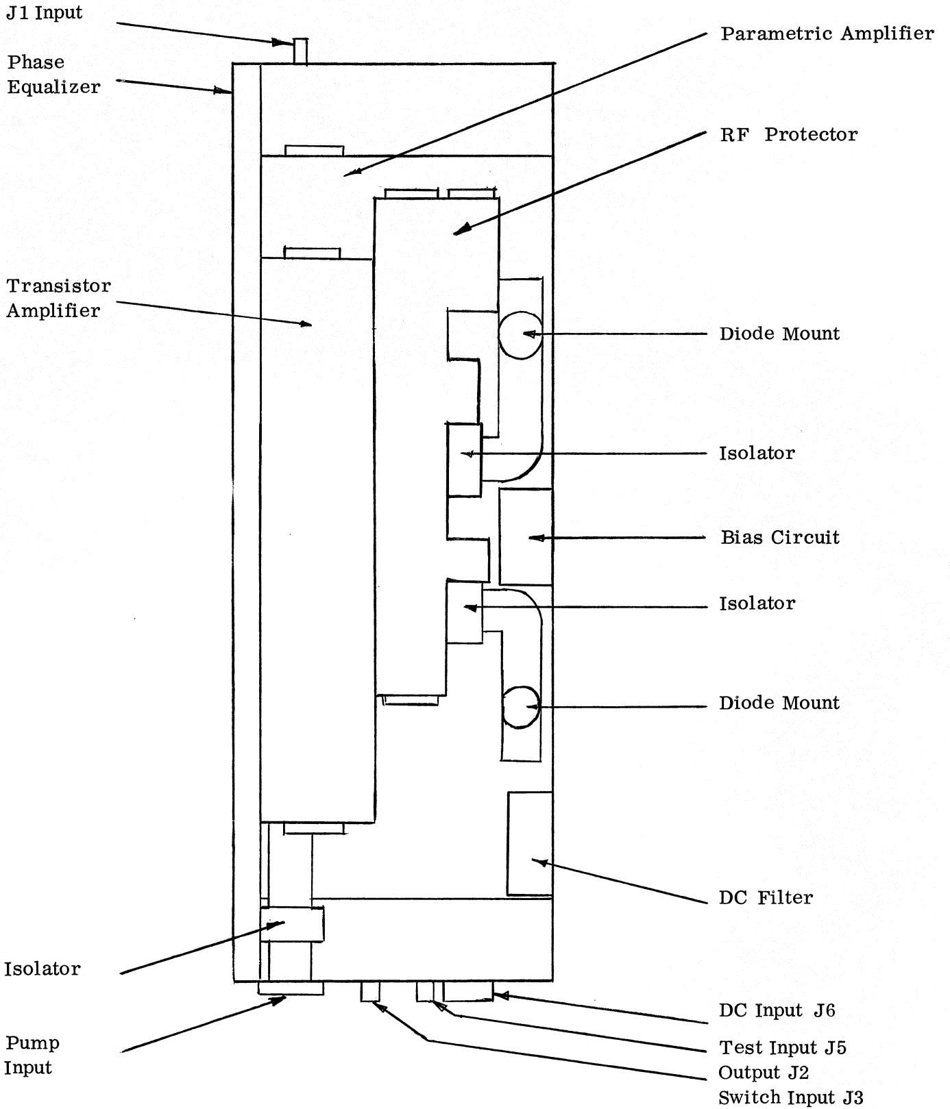
Figure 1 - Parametric Amplifier Unit
