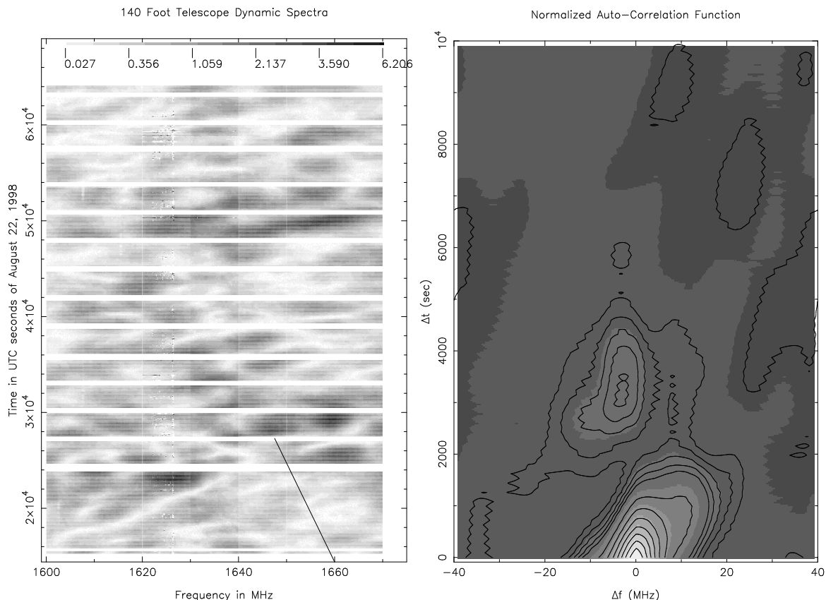
Figure 1. Dynamic spectra from the 140 Foot single dish data (a) and its normalized auto-correlation function (b). The line in the dynamic spectra indicates the direction of the fringes. The flux scale, in Jy, is given in the upper portion of (a). Interference from the Iridium satellites is clearly visible in (a). The contours in (b) are 0.0, 0.1, 0.125, 0.15, 0.175, 0.2, 0.3, 0.4, 0.5, 0.6, 0.7, 0.8, and 0.9.
