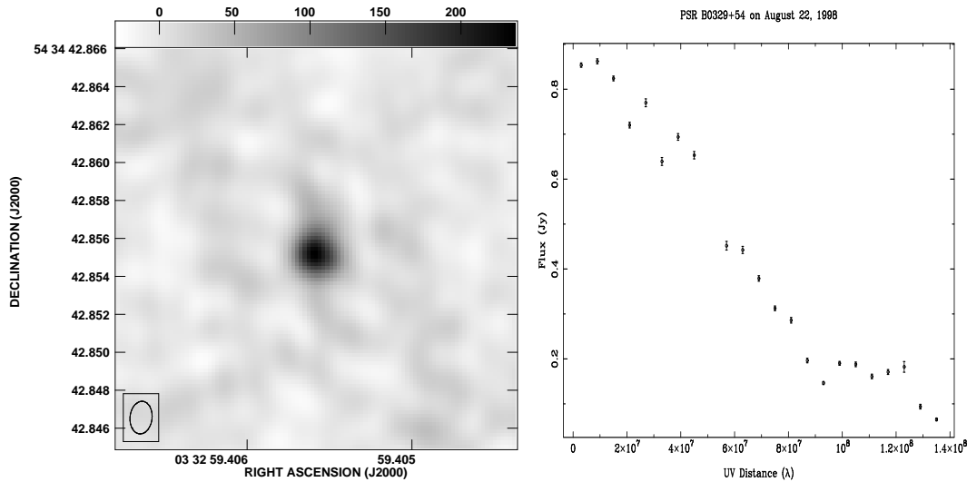
Figure 2. Image of PSR 0329+54 from the Space-VLBI observations during the interstellar fringing event (a). Flux vs. UV distance (b) determined from averaging within equally spaced radial bins in UV distance.
