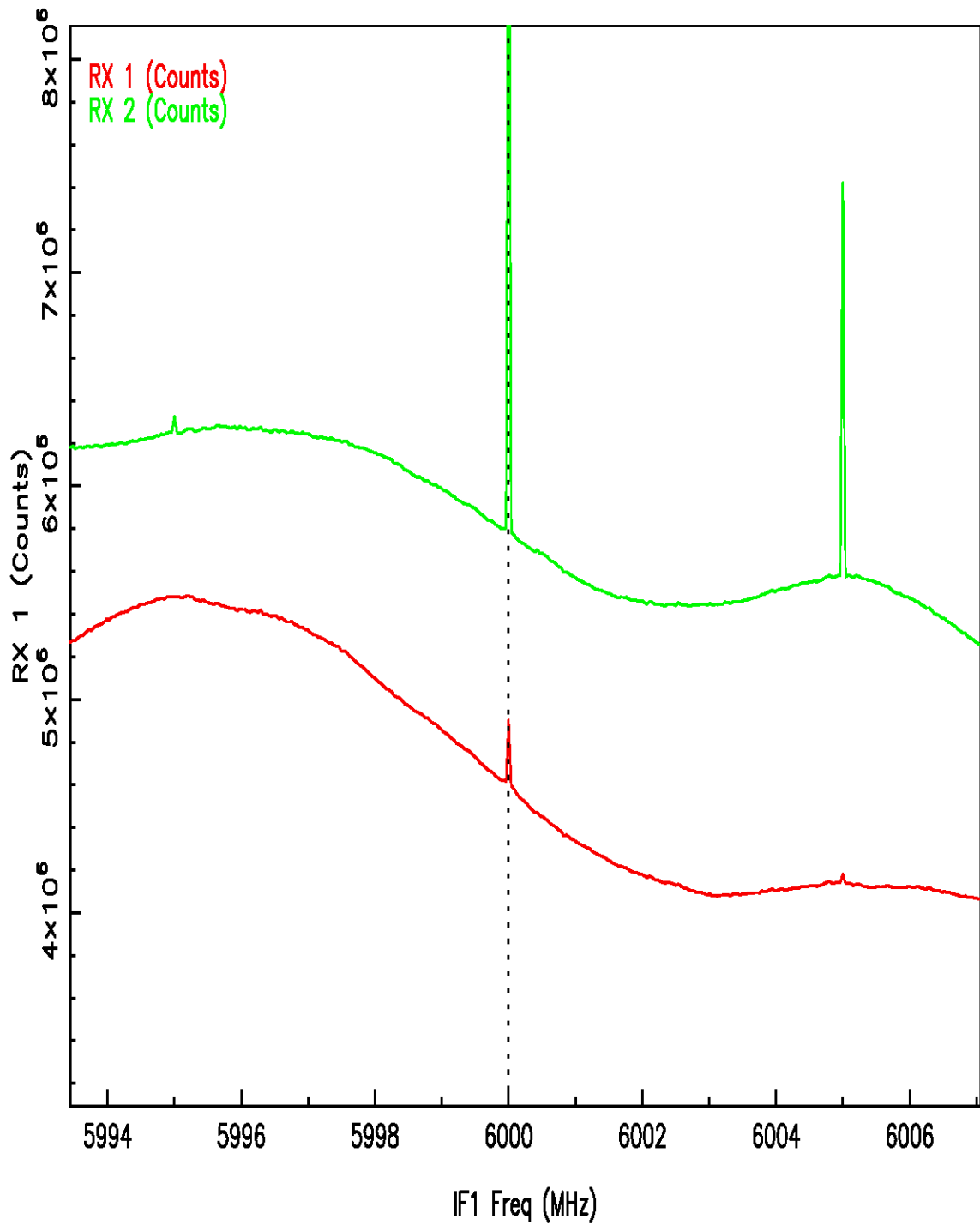
Figure 5: Strong interference located at channel 640 at IF3 = 195 MHz.
