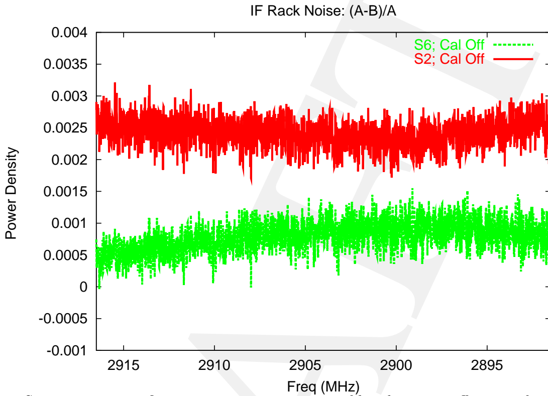
Figure 4: Same as previous figure, only central 25 MHz of bandwidth. Difference of average of two hours of scans and a second two hours of scans. The Optical Modem 1 data is red (top), Optical Modem 3 data is green (bottom).
