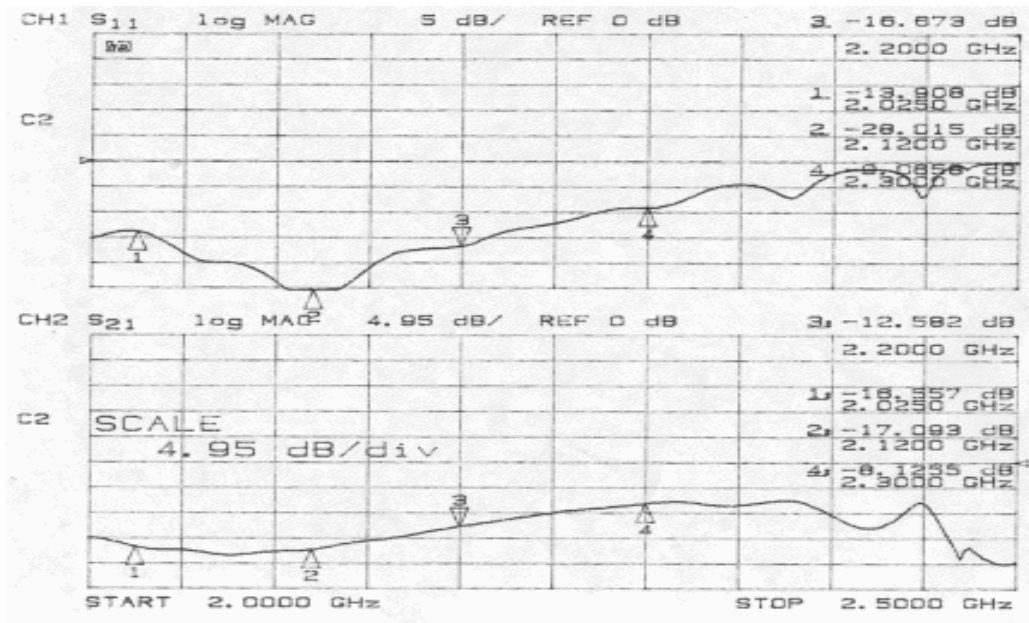
Figure 15: S Band Horn return loss (top) in the frequency range 2000 to 2500 MHz. The feed tuning ring is adjusted for maximum isolation in the uplink band. The rear port iris width is 3.275 in.
