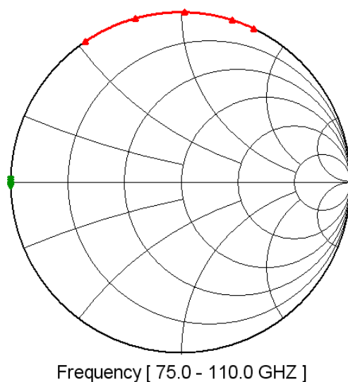
Fig. 2. WR-10 simulation. S_{11} with reference planes: D = 0 (red), D = 0.0202'' (green).
