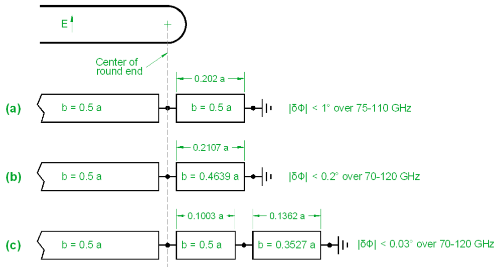
Fig. 4. Equivalent circuit models of the round-ended short-circuit. \delta\phi is the error in the phase of the reflection coefficient of the model relative to that of the QuickWave EM simulation.
