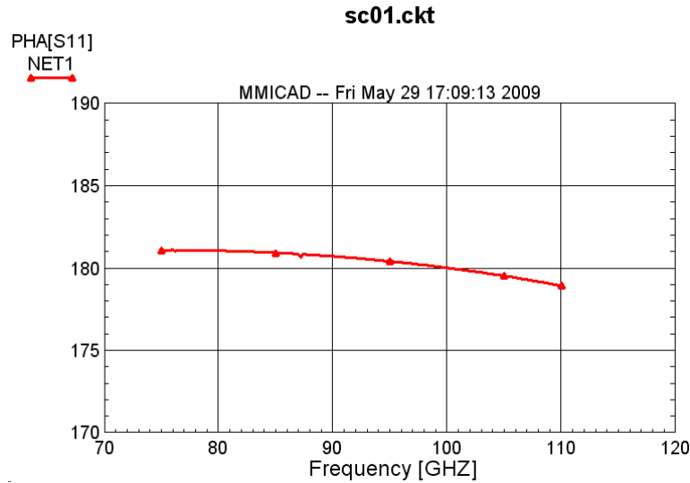
Fig. 3. Phase of S11 at plane D = 0.0202 a (red).
