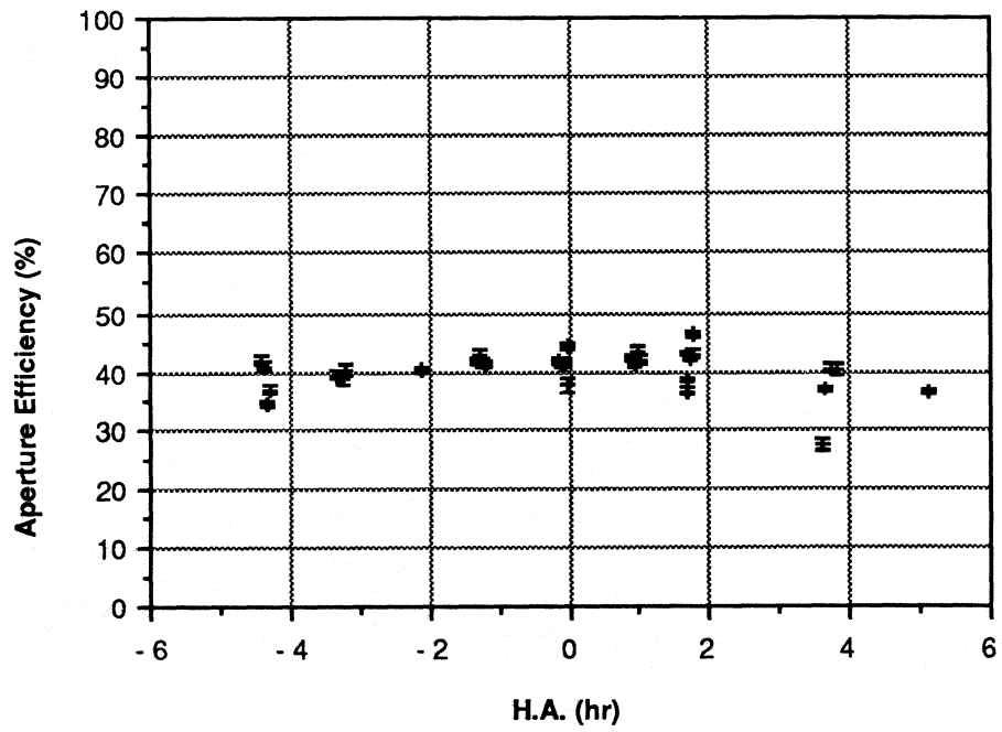
Fig. 1: XR Observations of VIRGO A
