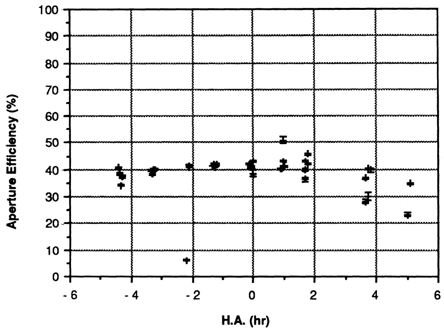
Fig. 2: XL observations of VIRGO A
