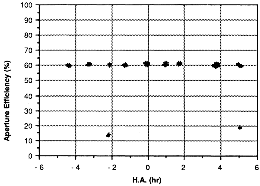
Fig. 3: SR observations of VIRGO A
