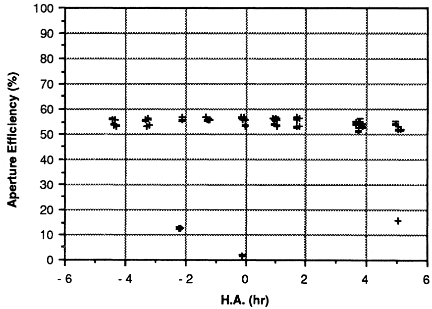
Fig. 4: SL observations of VIRGO A
