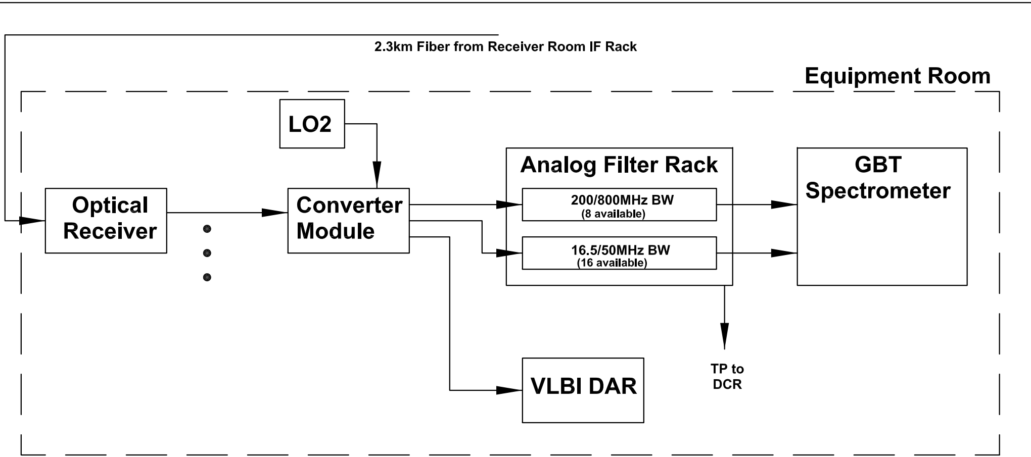
Figure 6-2 Equipment Room IF 4mm Receiver Project Book
