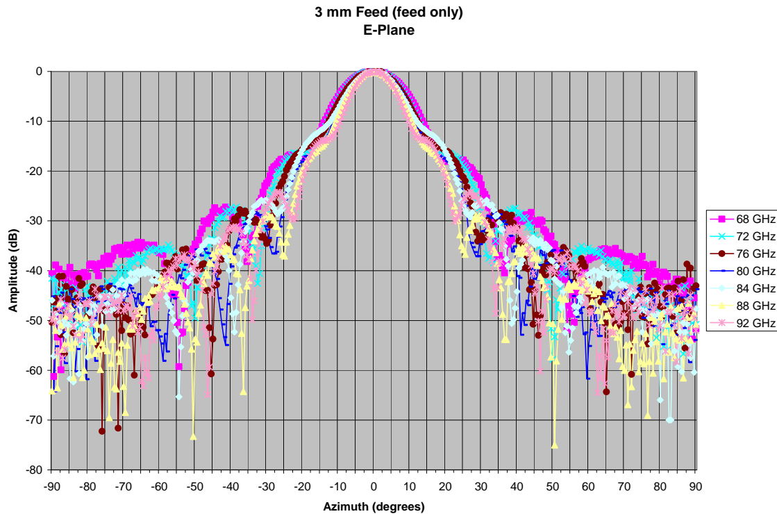
Figure 2: 3 mm Feed E-Plane Pattern
