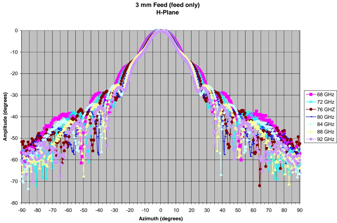
Figure 3: 3 mm Feed H-Plane Pattern
