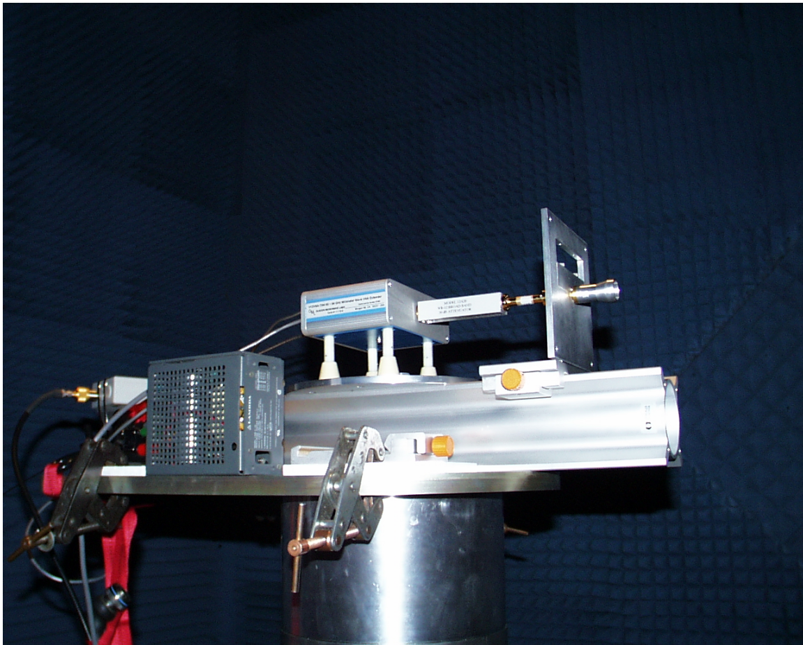
Figure 1: 3 mm Feed Test Setup (No Absorber)
