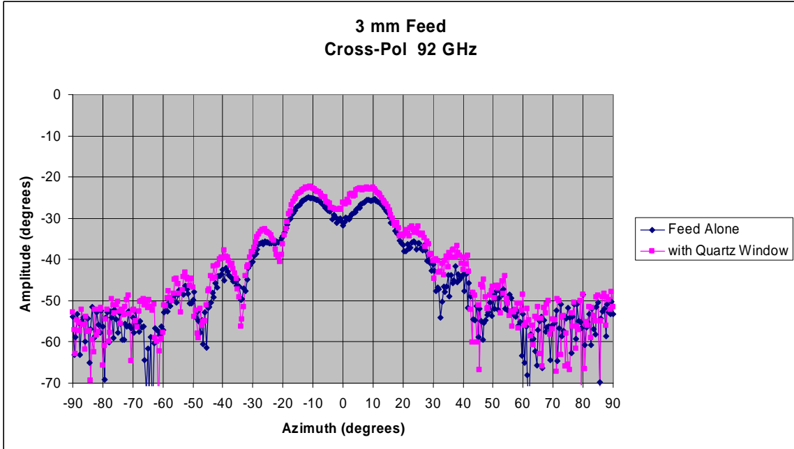
Figure 16: Cross-Pol, 92 GHz Comparison (with vs. without Quartz Window and IR Filter)
