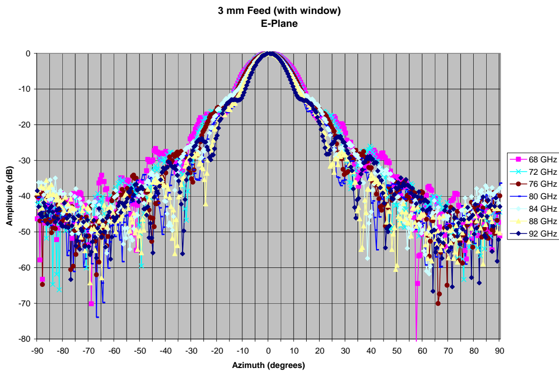
Figure 5: 3 mm Feed E-Plane Pattern (with Window)
