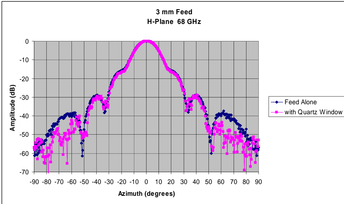
Figure 11: H-Plane, 68 GHz Comparison (with vs. without Quartz Window and IR Filter)
