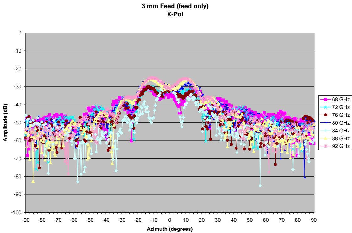
Figure 4: 3 mm Feed Cross-Polarization Pattern
