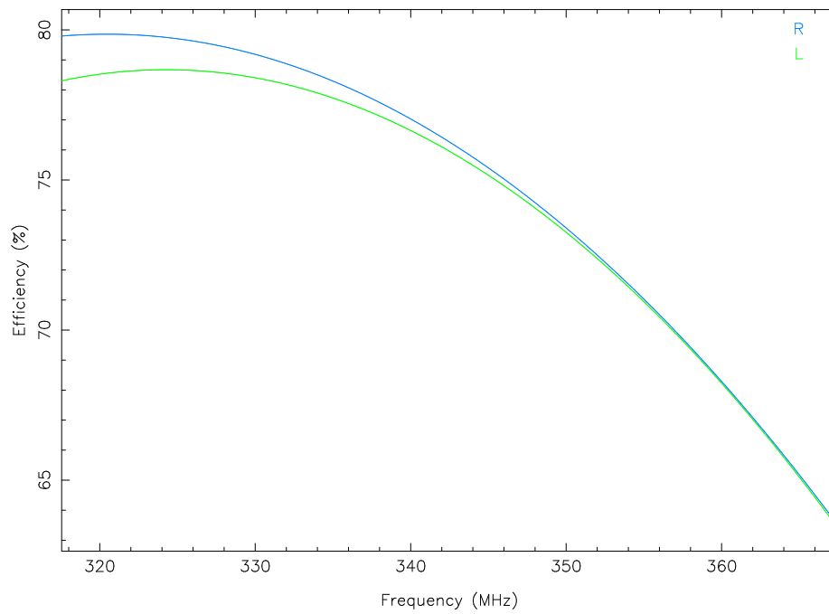
Figure 7: Fit to 3C295 LCP and RCP efficiency data, over the central 80% of the data in the previous plot.
