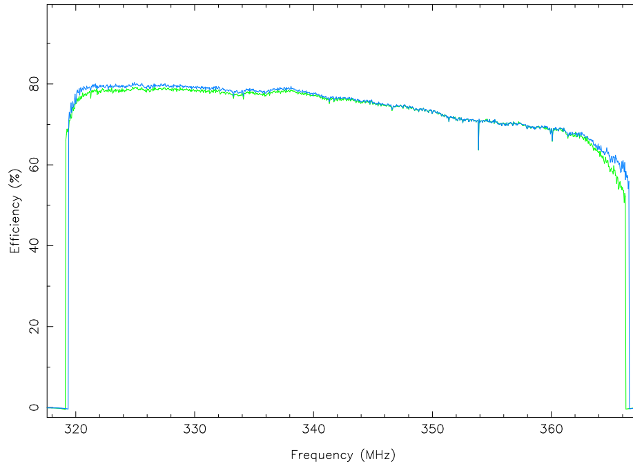
Figure 6: Measured GBT Efficiency based on observations of 3C295. This and the following plots are produced by glish scripts: setFluxes() ; updateEfficiency()
